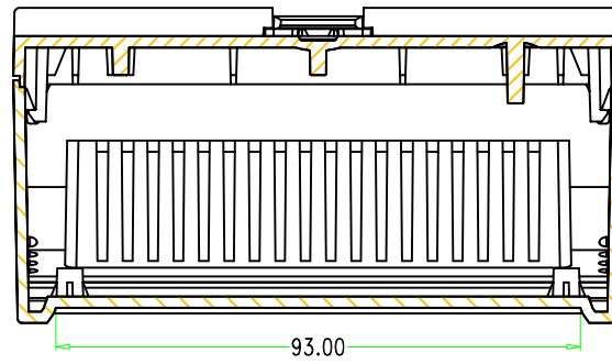
SEC B-B
