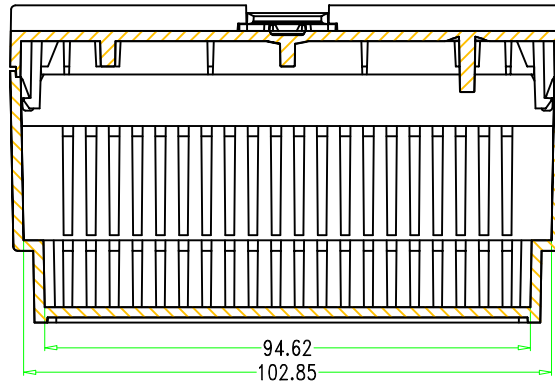
SEC B-B
