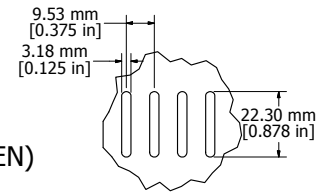
DETAIL KK
