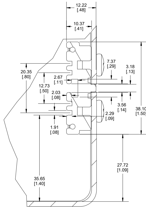
DETAIL C SCALE 1.3
