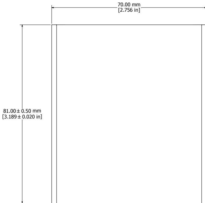
EXTRUSION
