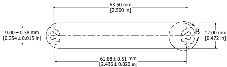
EXTRUSION
