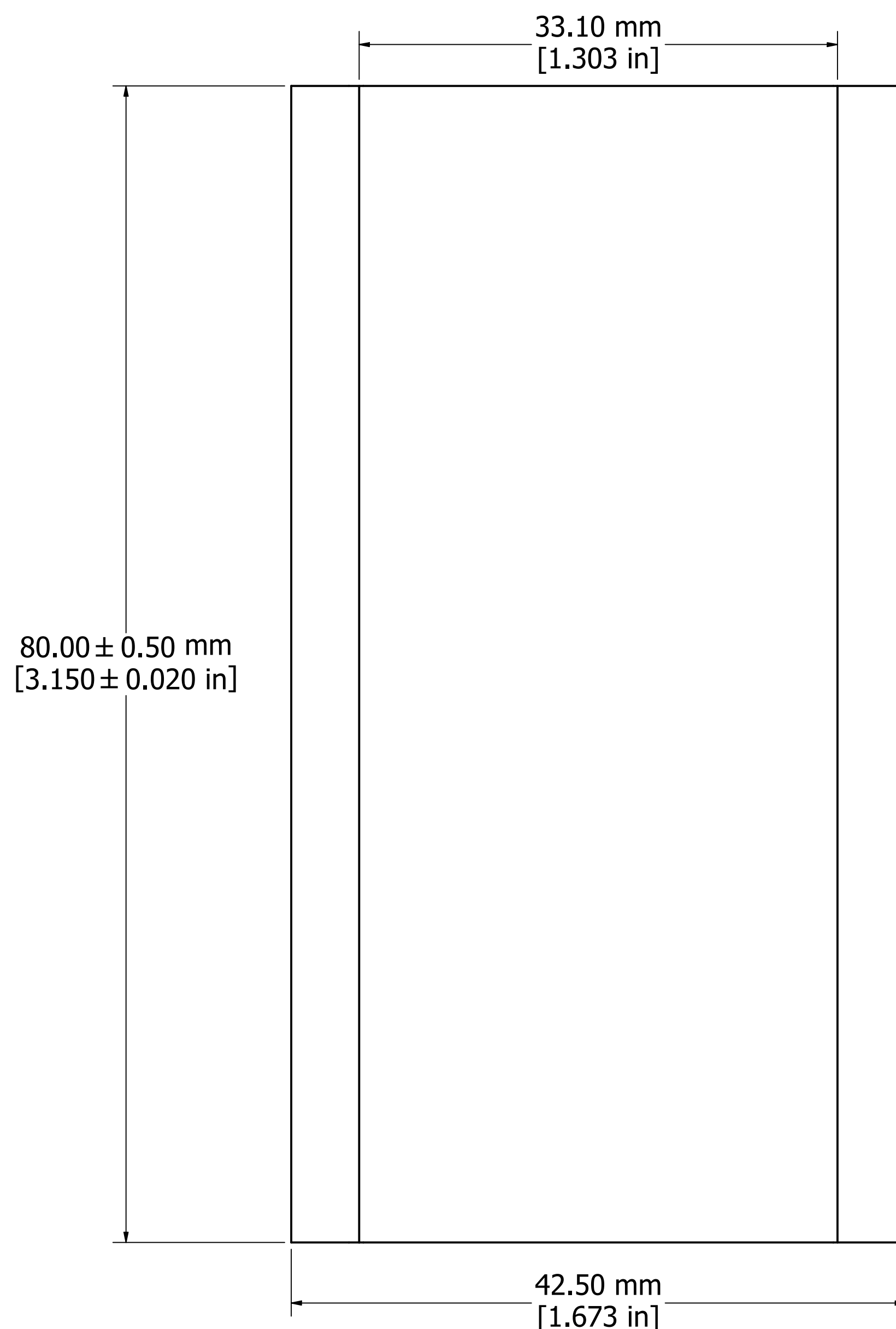
EXTRUSION PROFILE
