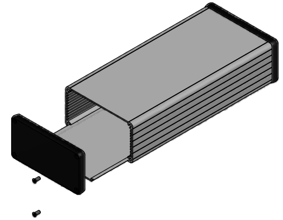
EXPLODED ASSEMBLY VIEW
