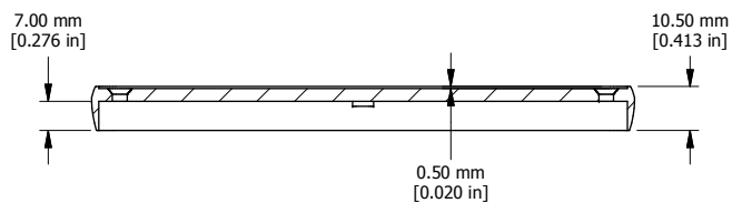
CLOSED BEZEL
