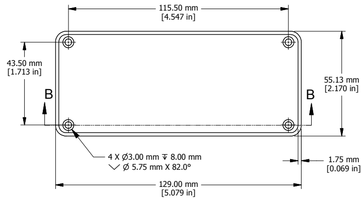
CLOSED BEZEL
