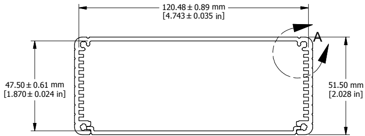
EXTRUSION
