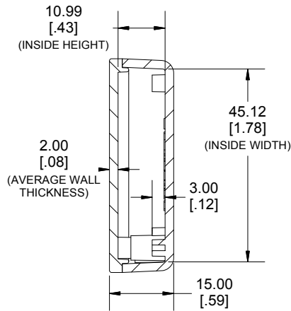
END VIEW SECTION B-B
