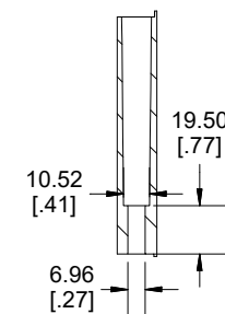
SECTION C-C MOUNTING HOLE
