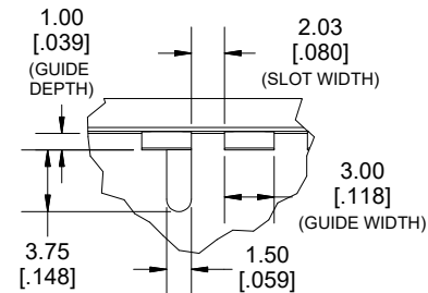
DETAIL D
