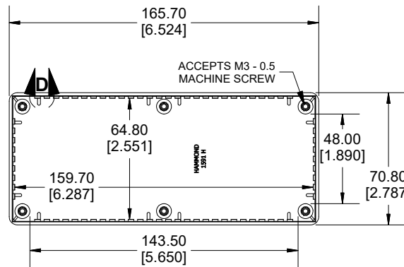
INSIDE BOX
