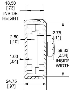
END VIEW SECTION A-A
