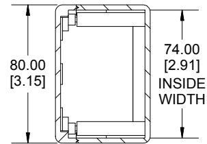
SECTION B-B END VIEW
