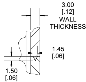
DETAIL C GROOVE
