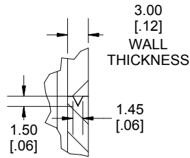
DETAIL D GROOVE
