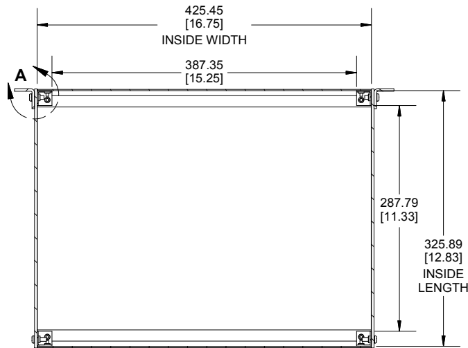
SECTION B-B INSIDE BOTTOM VIEW
