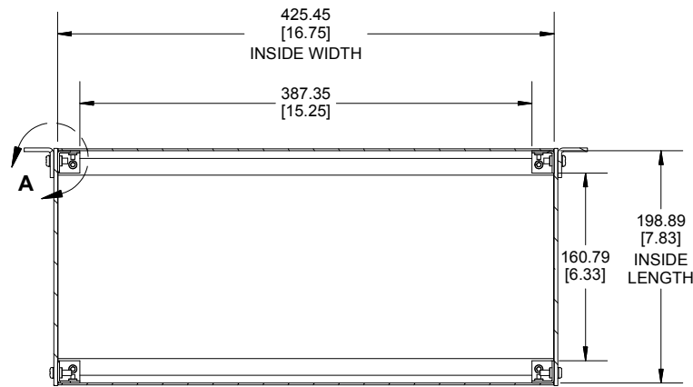
SECTION B-B INSIDE BOTTOM VIEW
