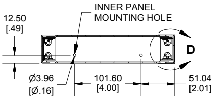
SECTION C-C INSIDE SIDE VIEW
