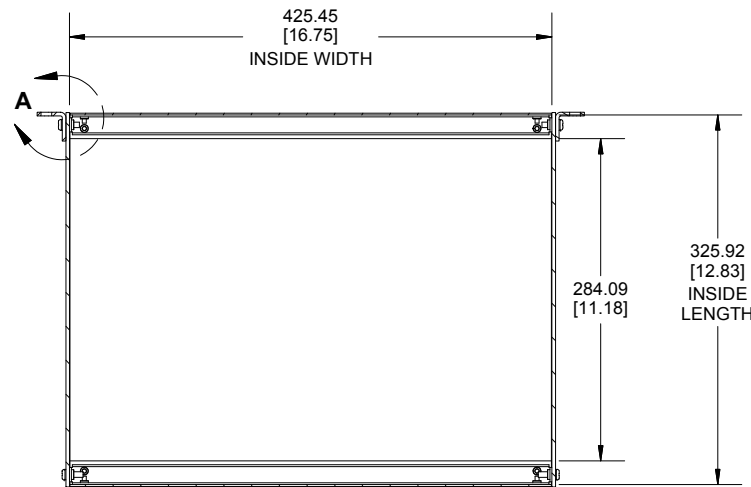
SECTION B-B INSIDE BOTTOM VIEW
