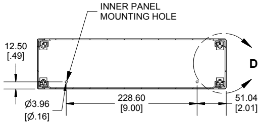
SECTION C-C INSIDE SIDE VIEW
