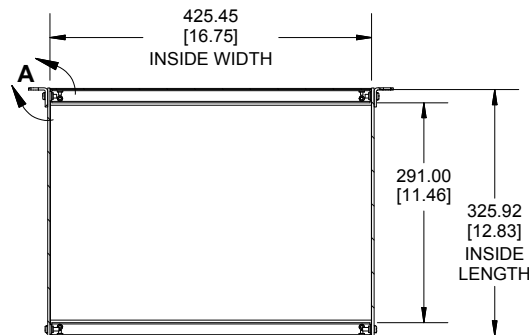
SECTION B-B INSIDE BOTTOM VIEW
