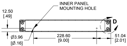
SECTION C-C INSIDE SIDE VIEW
