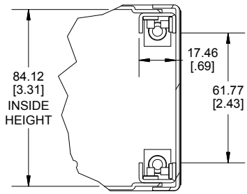
DETAIL D
