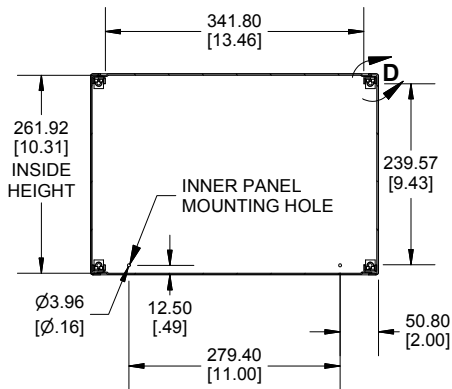
SECTION C-C INSIDE SIDE VIEW
