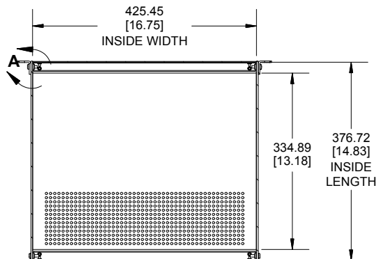
SECTION B-B INSIDE BOTTOM VIEW
