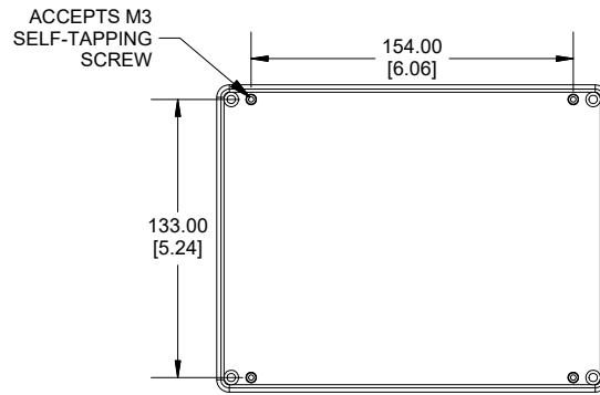
MOUNTING HOLES
