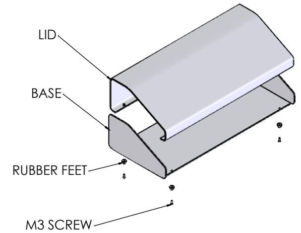
ISO VIEW 1:8
